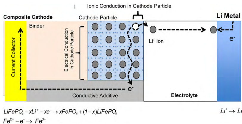
Fig. 3. Conduction phenomena in cathode particle ( \text{LiFePO}_4 ) during charge.
